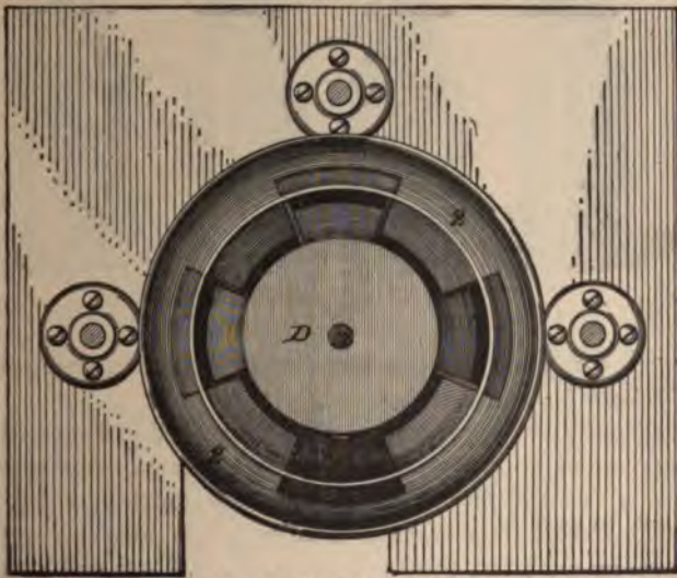
Laboratory Sampler.
